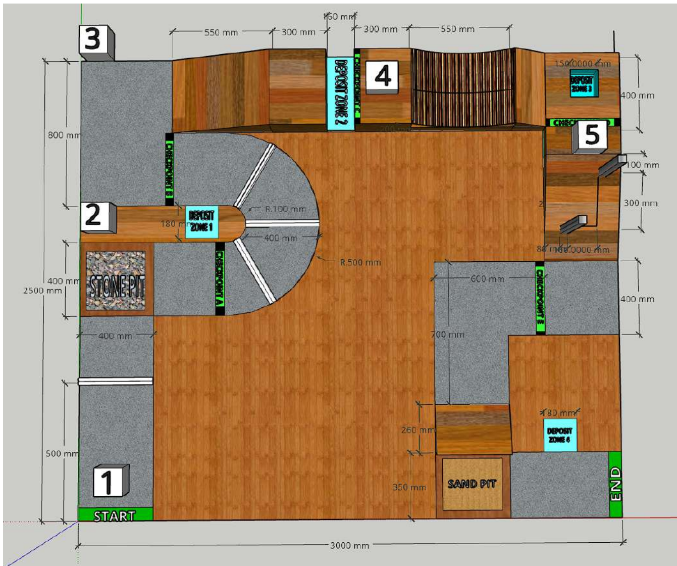
Fig.1 Top View
